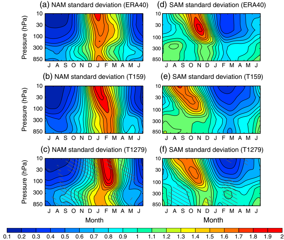
Figure 1. The standard deviation of the NAM and SAM indices as a function of season and pressure for (top) the ERA40 reanalysis and the IFS AMIP simulations at (middle) T159 and (bottom) T1279 resolutions. The hatching in the bottom panels indicates the areas where the difference of the standard deviation from the T159 case is significant at 10% confidence level based on F test.
