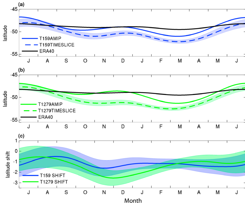
Figure 4. The mean locations of the surface westerly wind maximum in the SH from the AMIP (solid line) and time-slice (dashed line) simulations by the IFS at (a) T159 and (b) T1279 resolutions, together with the ERA40 reanalysis (black line). (c) The degrees of shift in the surface westerly winds in the time-slice simulations with T159 (blue line) and T1279 (green line) resolutions, respectively. The shading indicates the 95% confidence interval based on Welch's t test.
