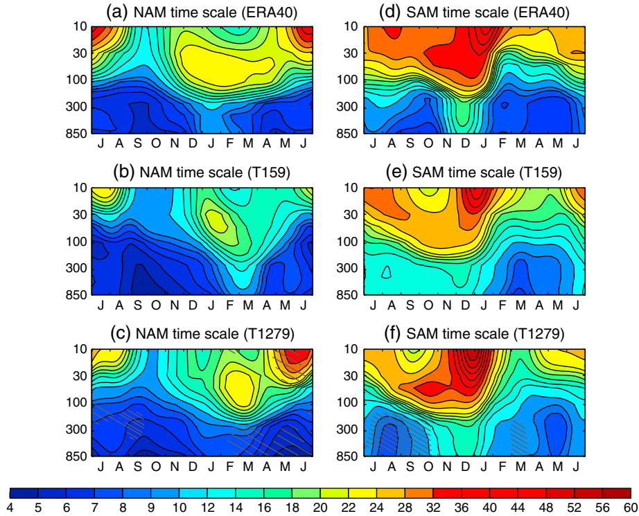
Figure 2. The e -folding time (days) of the NAM and SAM indices as a function of season and pressure for (top) ERA40 and IFS AMIP simulations at (middle) T159 and (bottom) T1279 resolutions. The hatching in the bottom panels indicates the areas where the difference of the AM time scale between the two resolutions is greater than the uncertainty of the time scale due to one standard deviation of the autocorrelation function of the AM index estimated following Gerber et al. [2008a, 2008b].
